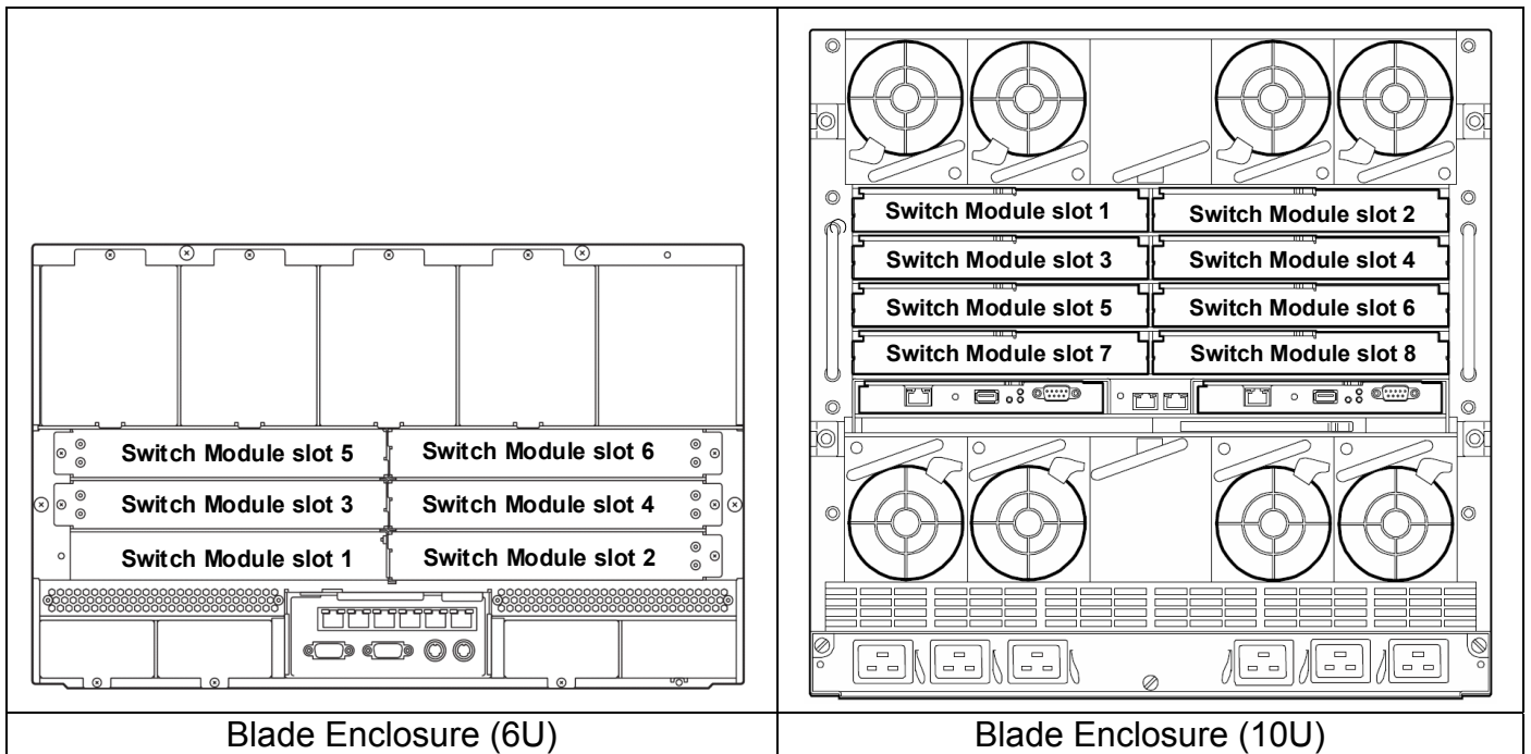
Rear View
